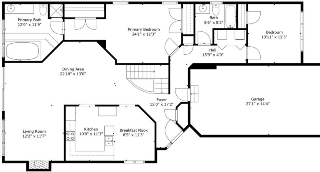
Floor 2
